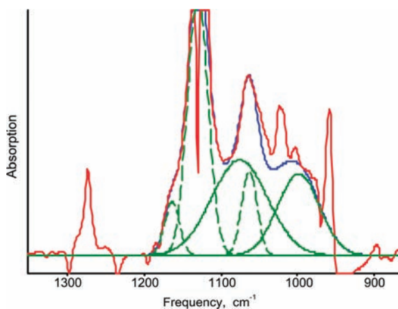
Figure 4. Deconvolution (green), with summation (blue), of the spectrum of 2·H{Cl 11 } with absorptions of {Cl 11 } - anion subtracted (red) showing broad bands at 1075 and 985 cm -1 assigned to bridging proton vibrations (solid green).
